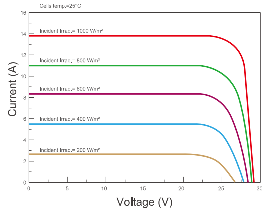
Current-Voltage & Power-Voltage Curves (RMHT40/320F2)
