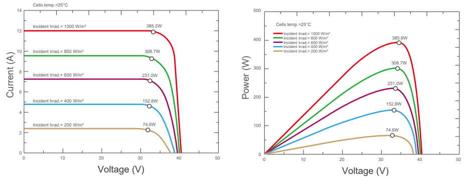
Current-Voltage &amp; Power-Voltage Curves (RMHT54/385GW1)
